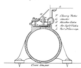
Cross section of Pipe Showing roller P which closes the Valve, and the Heater G which seals the edge, air-tight ready for next train
