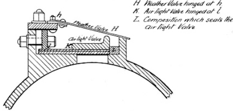
Cross Section of Pipe with Valve
